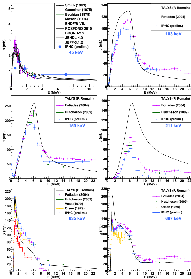
Fig. 5: Cross-sections of (n, n'\gamma) reactions on ^{238}\text{U} as a function of incident neutron energy.
