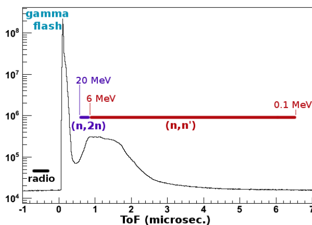
Fig. 2: Part of the ToF distribution, in one HPGe detector.
